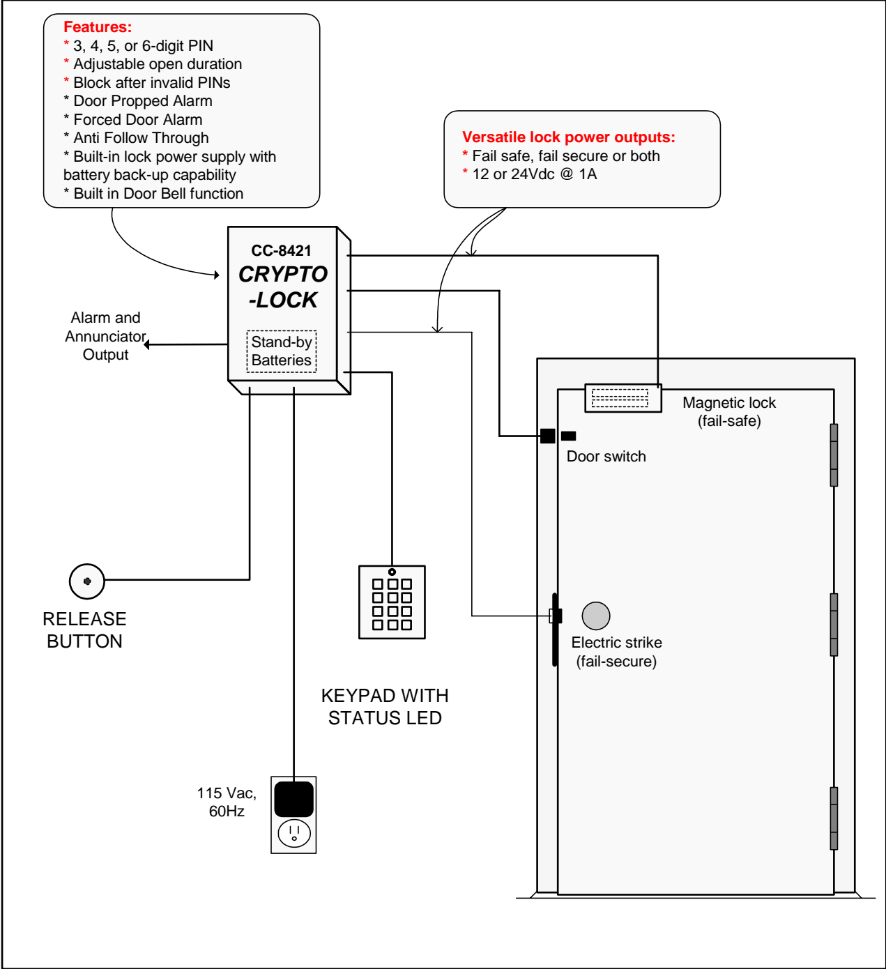
Figure 1-2, Typical Application of the Model CC-8421 Access Controller
